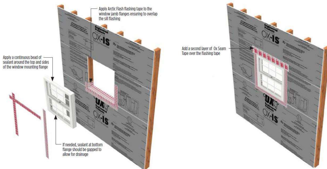
Figure 4. Typical Window Flashing Detail
